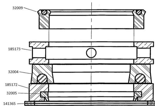
RAM SHAFT SEAL ASSEMBLY
